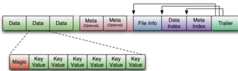
Figure 13. HFile V1 Format
